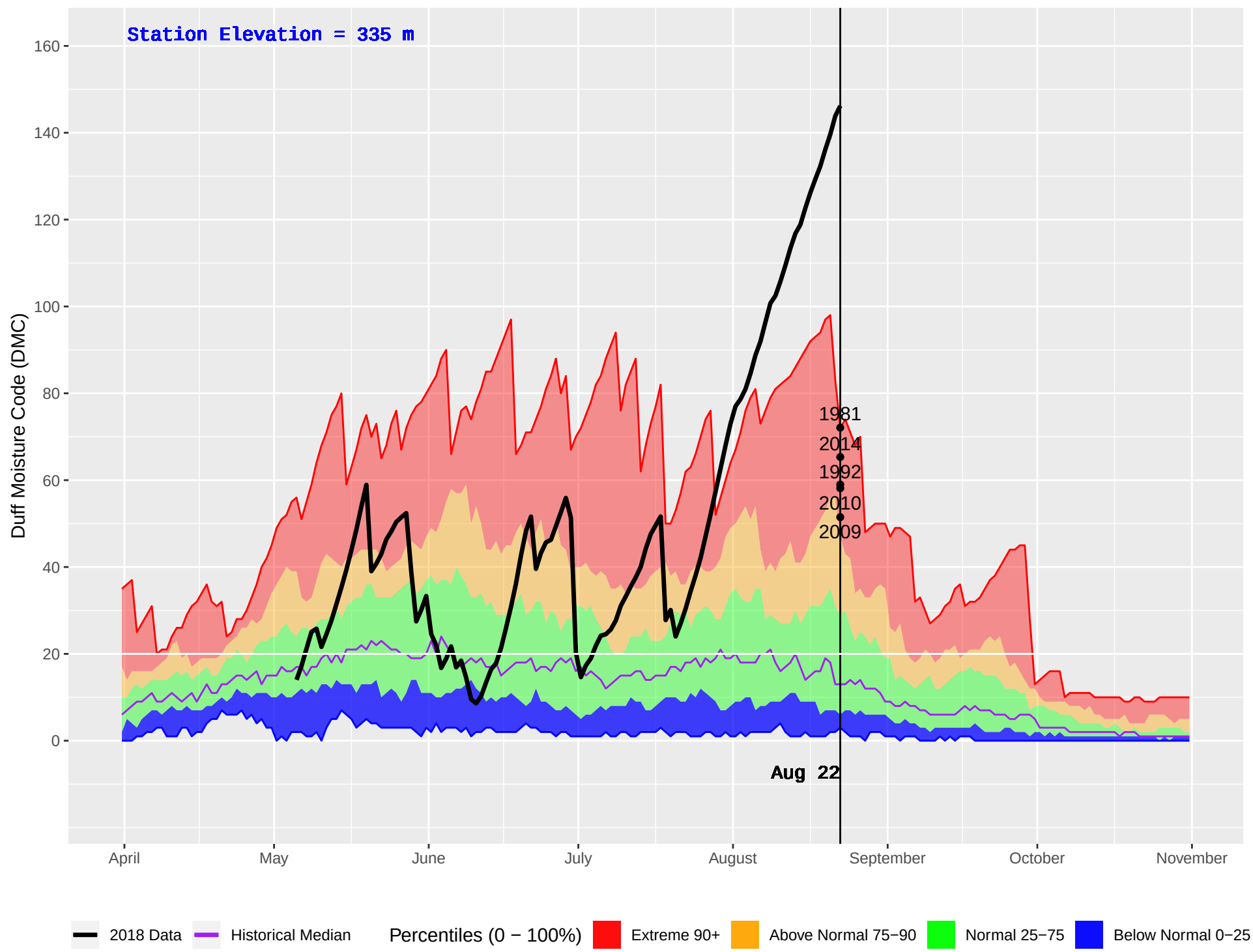
KISPIOX HUB (428) : Historical (1970–2016) and Current (2018) Daily Duff Moisture Code (DMC)
