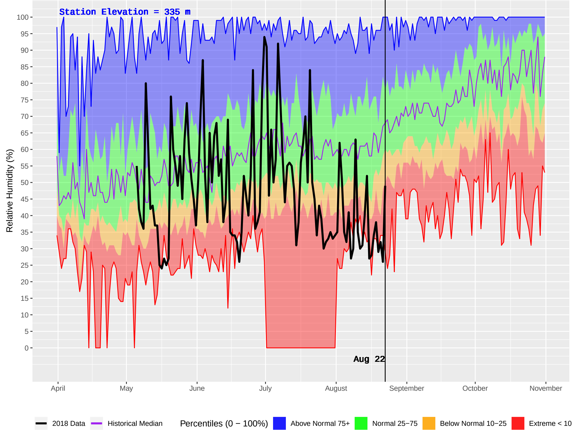
KISPIOX HUB (428) : Historical (1970–2016) and Current (2018) Daily Relative Humidity
