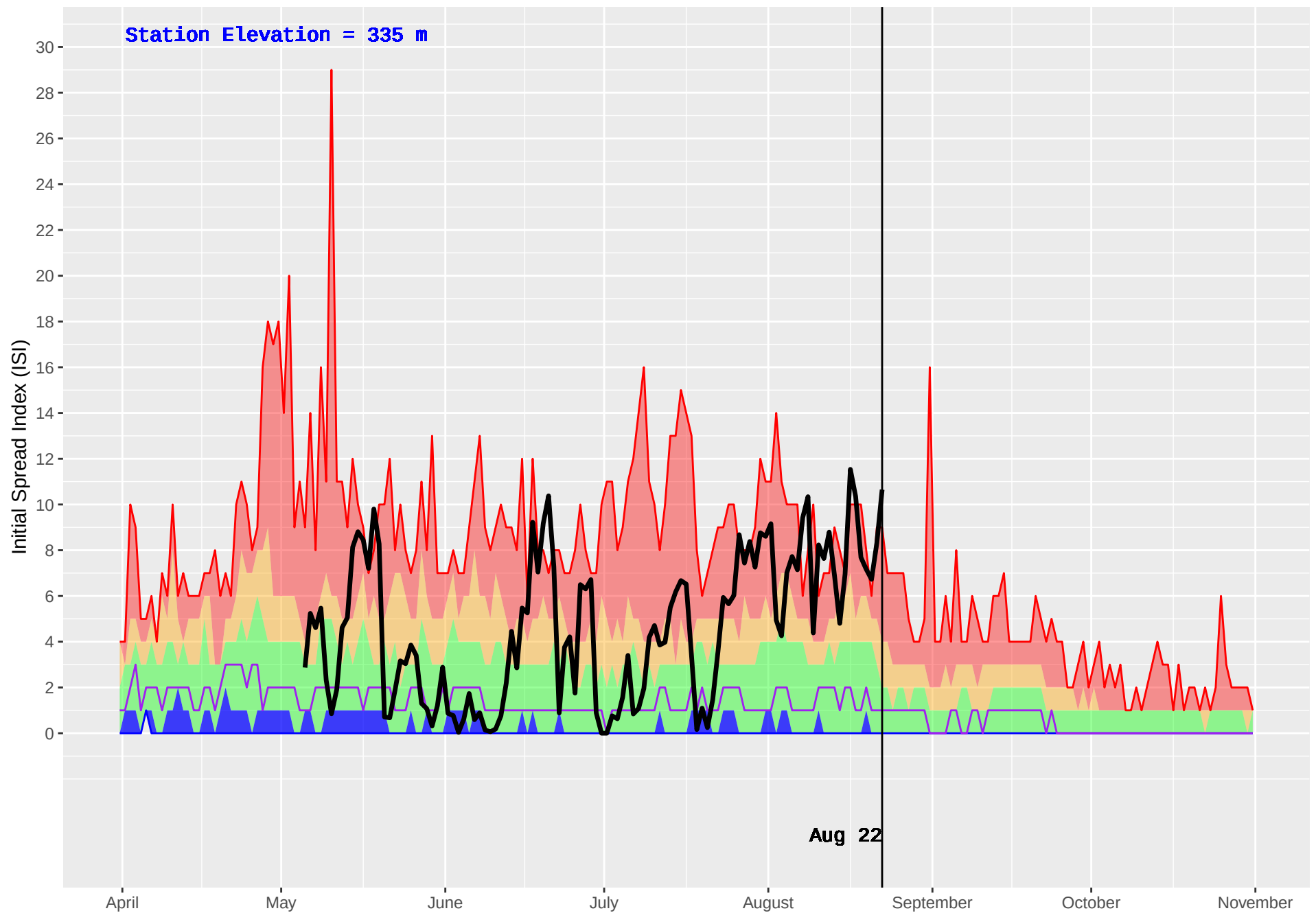
KISPIOX HUB (428) : Historical (1970–2016) and Current (2018) Daily Initial Spread Index (ISI)
