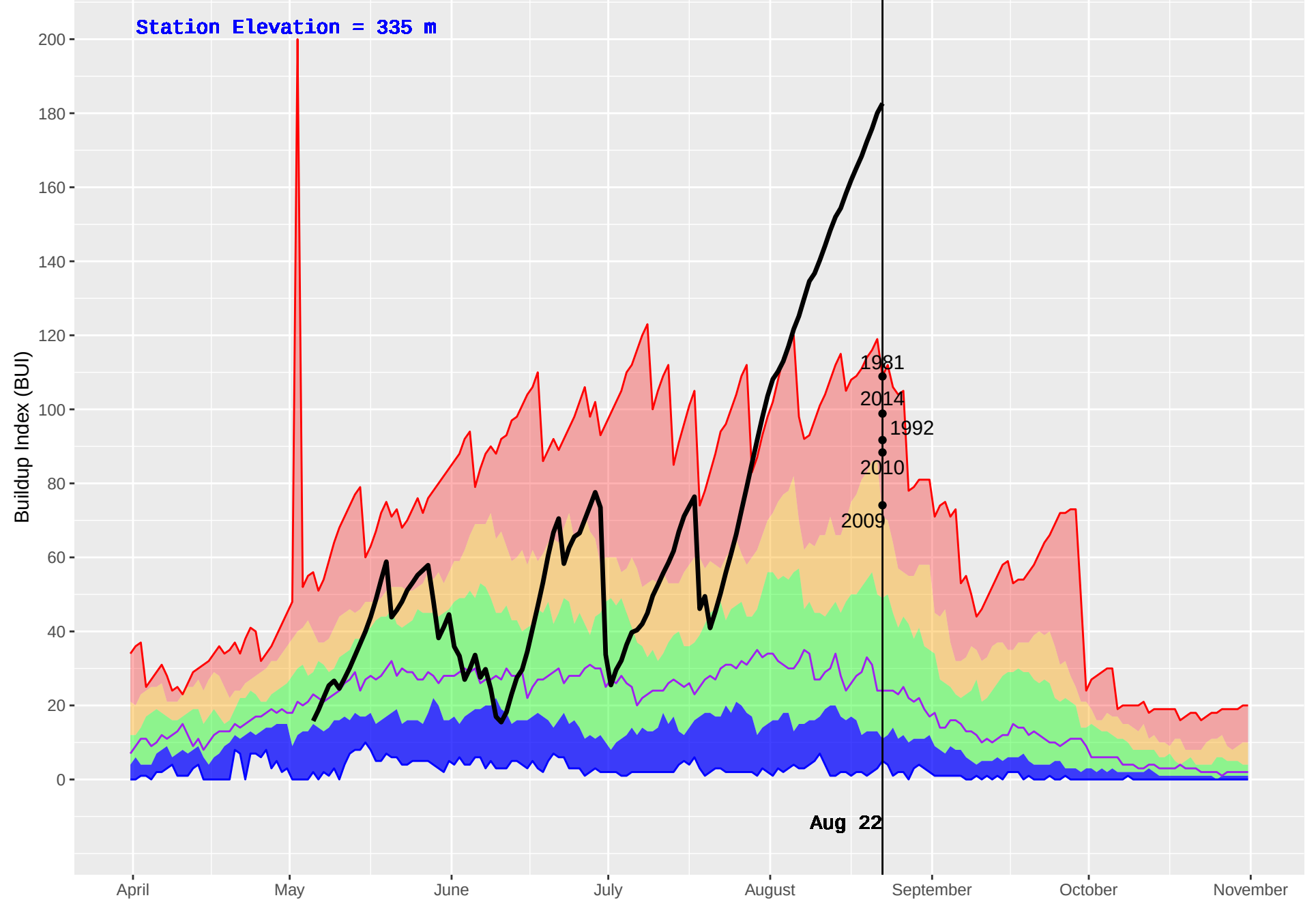
KISPIOX HUB (428) : Historical (1970–2016) and Current (2018) Daily Buildup Index (BUI)
