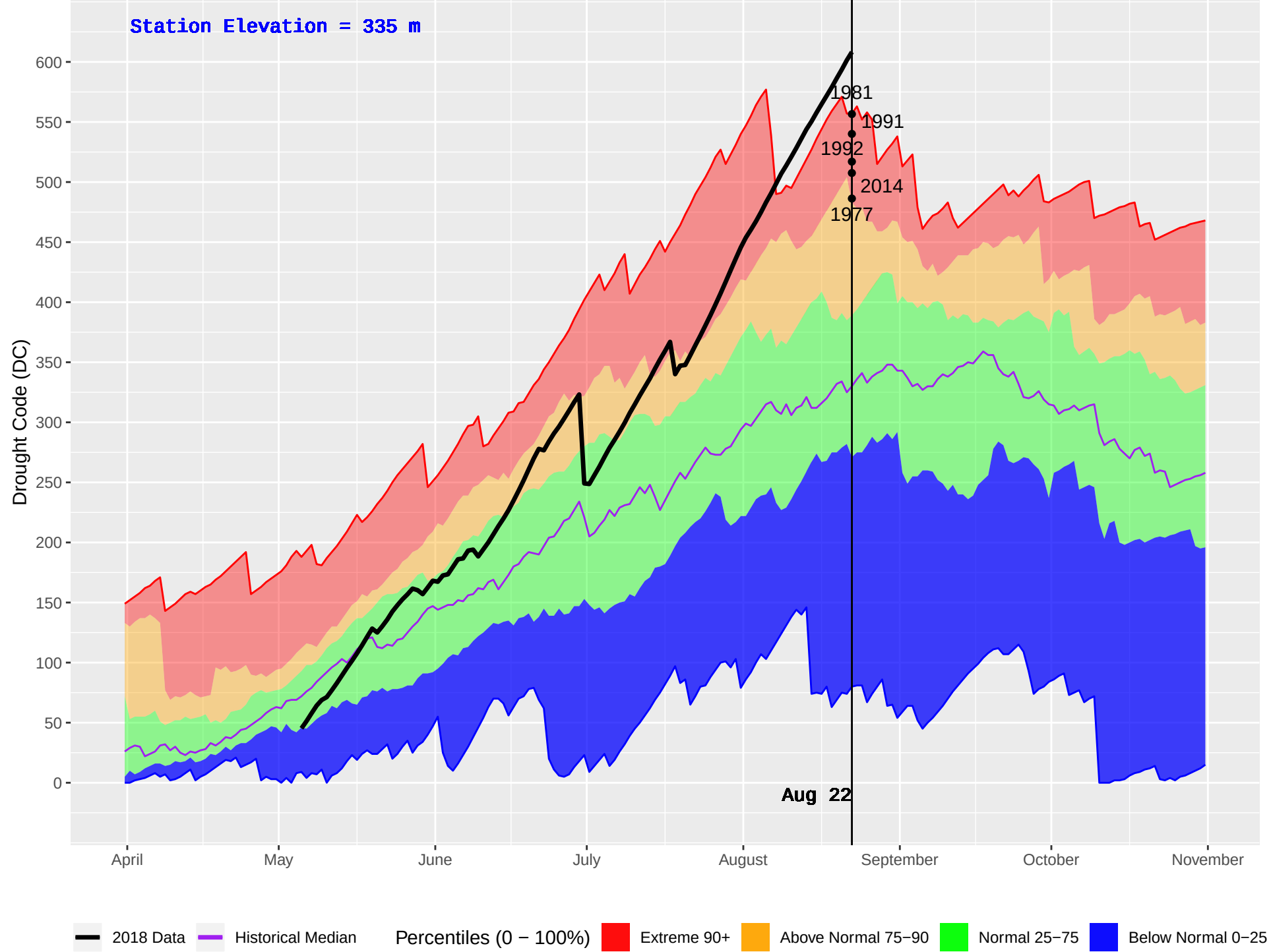
KISPIOX HUB (428) : Historical (1970–2016) and Current (2018) Daily Drought Code (DC)
