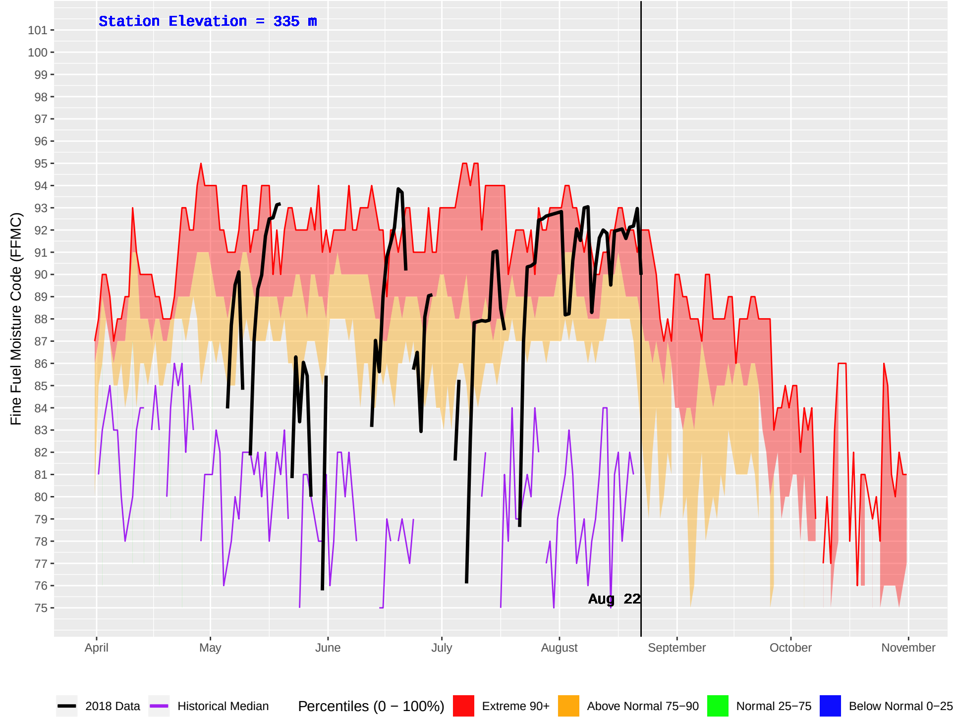
KISPIOX HUB (428) : Historical (1970–2016) and Current (2018) Daily Fine Fuel Moisture Code (FFMC)
